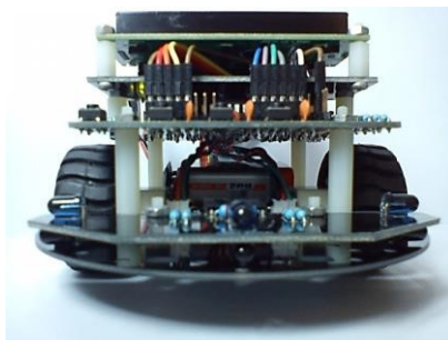
Figure 2. Mobile robot from side view.
