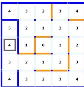
Figure 16. Simulation search path to cell (2,2)
