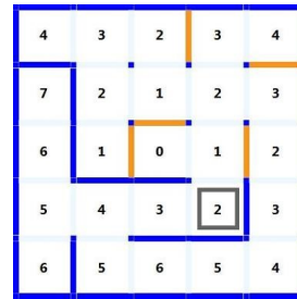
Figure 20. Simulation search path to cell (2,2)
