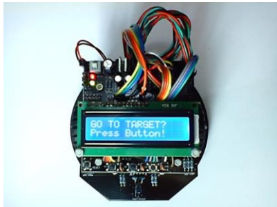
Figure 5. Mobile robot from above view.
