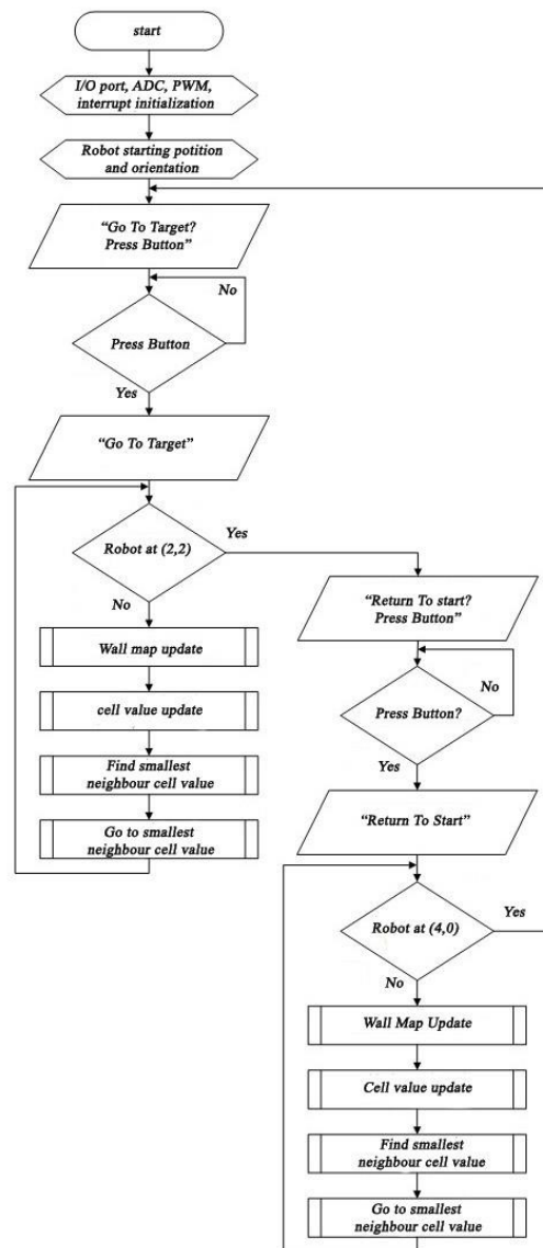
Figure 4. Flowchart of the main program
