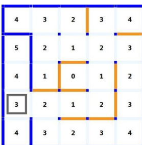
Figure 17. Simulation search path to cell (2,2)
