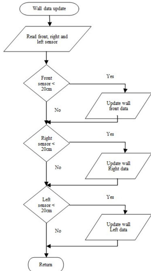
Figure 9. Flowchart for updating wall location at each cell
