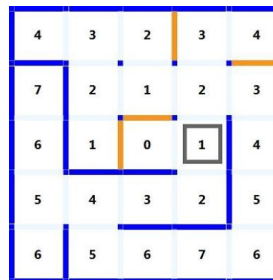
Figure 21. Simulation search path to cell (2,2)
