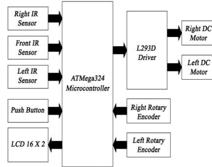
Figure 3. Block diagram of mobile robot.
