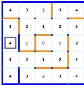
Figure 14. Simulation search path to cell (2,2)
