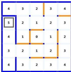
Figure 15. Simulation search path to cell (2,2)
